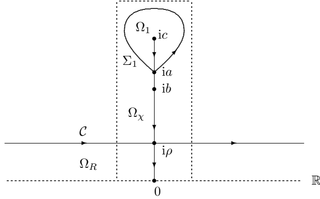
FIGURE 3. Jump contour \Sigma^{(2)} in \mathbb{C}^+ (without the \mathbb{T}_j 's)
