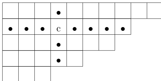
FIGURE 30. A cell c in the shape of the partition \lambda = (10, 8, 7, 5, 3) \vdash 33 with a(c) = 4 , a'(c) = 3 , l(c) = 2 and l'(c) = 1 .
