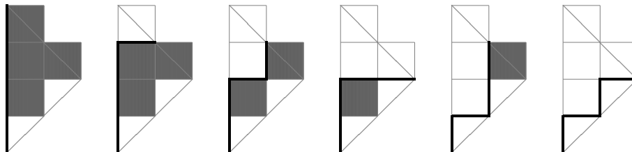
FIGURE 15. All type B Catalan paths of length 2.
