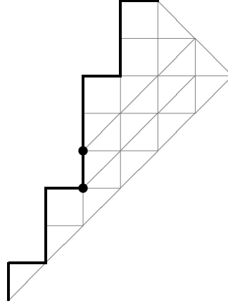
FIGURE 16. A Catalan path of type B_6 .
