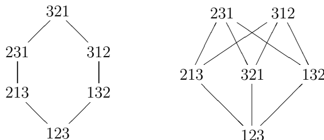
FIGURE 18. \text{Weak}(A_2) and \text{Abs}(A_2) .
