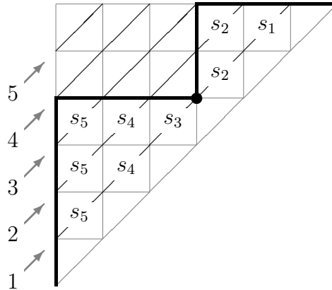
FIGURE 23. A Catalan path of length 6 with cells labelled by simple transpositions.
