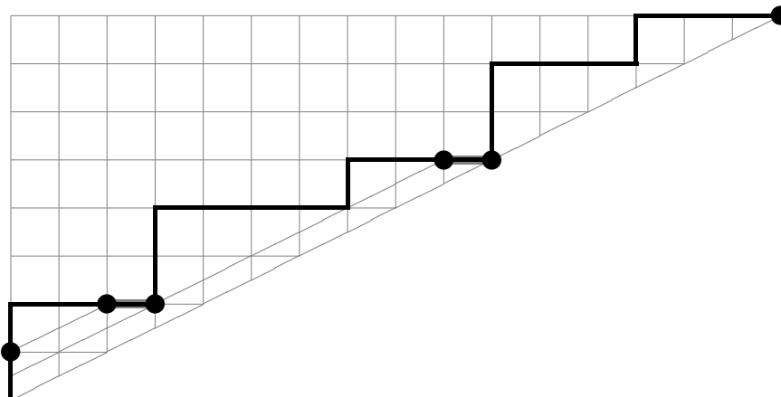
FIGURE 13. The dissection of a 2-Catalan path of length 8 into three 2-Catalan paths of lengths 1, 3 and 3 respectively.
