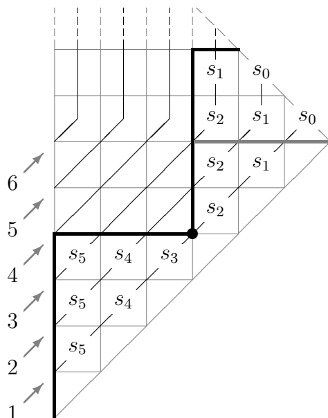
FIGURE 24. A Catalan path of type B_6 with cells labelled by simple transpositions.
