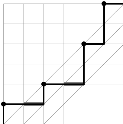
FIGURE 17. The lattice path from (0,0) to (6,6) which is mapped to to Catalan path of type B_6 shown in Figure 16.
