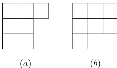
FIGURE 28. The shape of the partition \lambda = (3, 2^2) \vdash 7 and of its conjugate partition \lambda' = (3^2, 1) \vdash 7 .
