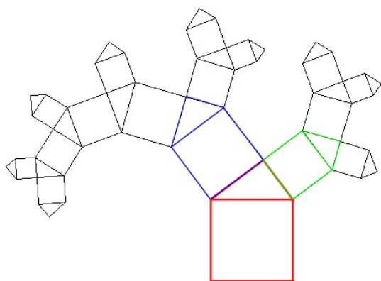
Abb. 4.13: Pythagorasbaum
