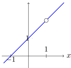
Abb. 5.16: f(x) = \frac{x^2 - 1}{x - 1}
