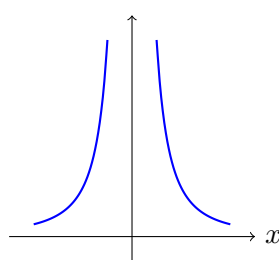
Abb. 5.17: f(x) = \frac{1}{x^2}
