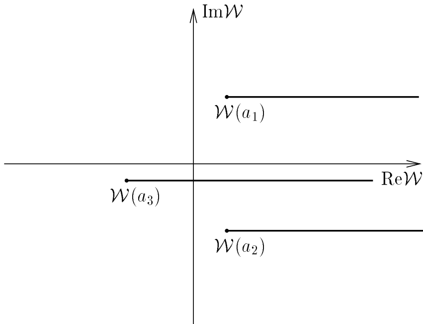
Figure 11: Vanishing cycles of the massive \Phi^4 LG theory in the \mathcal{W} plane.
