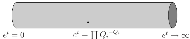
Figure 1: The classical and quantum moduli space of one-parameter models.
