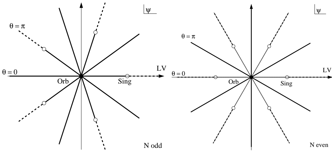
Figure 6: The N -fold cover of the Kähler moduli space, e^t = (-N\psi)^N . Relation (92) says that we can move straight through the orbifold point. For N odd (here 5) the two slices, at \theta = 0 and \theta = \pi , are connected at the orbifold point. For N even (here 6) the two slices, at \theta = 0 and \theta = \pi , remain disconnected.
