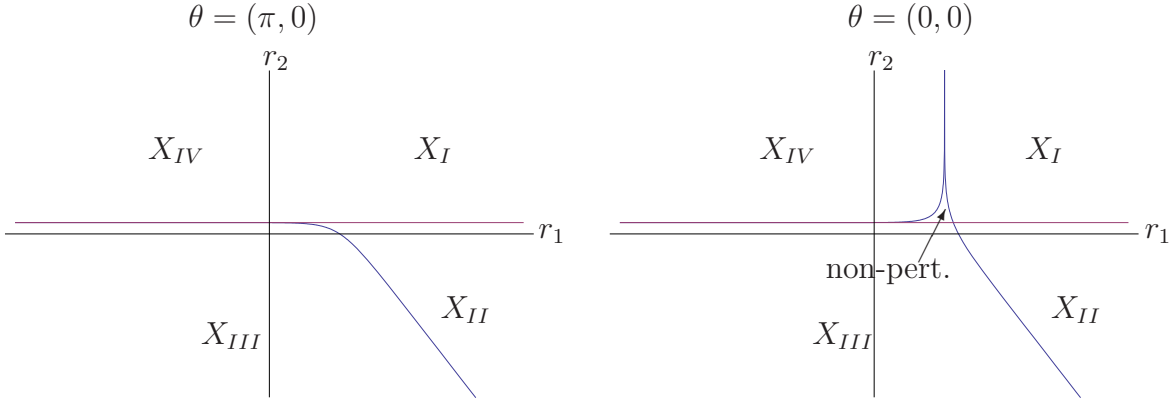
Figure 5: The slices \theta = (\pi, 0) resp. \theta = (0, 0) divide the moduli space in distinct sectors.
