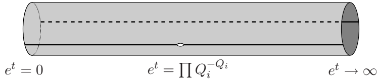
Figure 4: The slices of the moduli space in the presence of an orientifold. One slice connects the large volume and the 'small' volume point (sometimes Gepner point).
