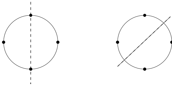
Figure 8: Branes in an \mathbb{Z}_4 orbifold and possible inequivalent reflection planes: Either two or no branes are invariant under the parity.
