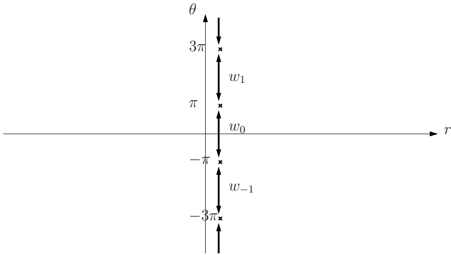
Figure 3: Windows for the grade restriction rule. Here \mathcal{S} is odd.
