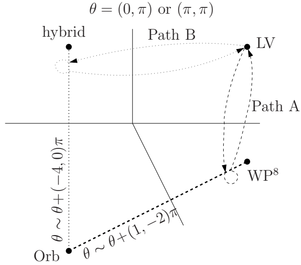
Figure 9: In the two-parameter model, Example 2, the two slices, \theta = (0, \pi) and (\pi, \pi) , are connected along the (dashed) line at infinity in phases II and III. This is due to the vacuum expectation value of the field x_6 . As a consequence, two large volume limits are connected via Path A in the moduli space. Path B induces a non-trivial monodromy but returns to the original large volume point.
