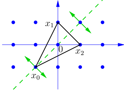
Figure 4: Symmetry of the toric polytope defining \mathbb{P}^2 .
