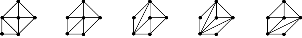
Figure 1: The five different triangulations of the toric \mathrm{dP}_2 base.
