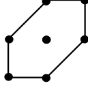
Figure 2: The points of the polyhedron of the \text{dP}_3 base.
