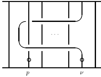
Fig. 3: Pictorial presentation of Lemma 6. The picture contains m + 2g strands, one for every puncture and two for every handle. It shows the action of \eta_{\nu p}, 1 \leq \nu \leq m, \nu < p \leq m + 2g on states. Over- and undercrossings correspond to factors R, R^{-1} and the open circle on a line s means multiplication with v_{K_s}^{-1} .
