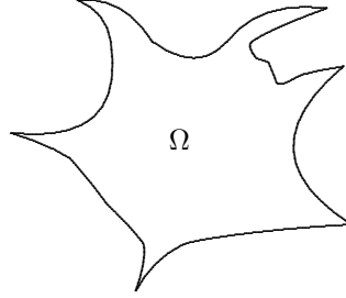
FIGURE 1. A quasi-convex domain.
