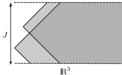
Two wedges in FRW spacetime
