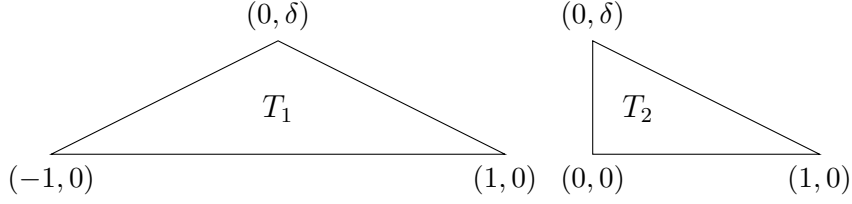
FIGURE 3.2. The triangles T_1 and T_2 from Example 3.1.
