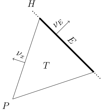
FIGURE 2.1. Geometry of the triangle T from Lemma 2.1 and Lemma 2.2.
