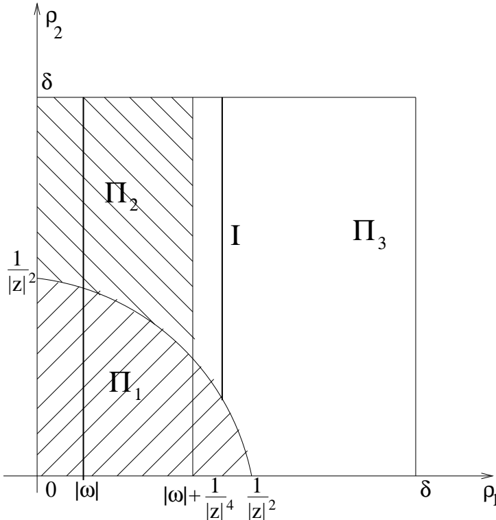
Figure 1: The case |\omega| - 1/|z|^4 < 0 .
