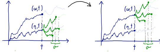
FIGURE 2. The left hand side of (3.2) corresponds to averaging the function c over the stopped paths on the left picture, the right hand side to averaging the function c over the stopped paths on the right picture.
