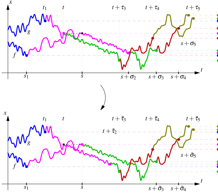
Fig. 1 We show a potential stop-go pair. In the top picture, we show the pair ((f, s_1, s), (g, t_1, t)) with corresponding stopping times \tau_3, \dots, \tau_5 and \sigma_2, \dots, \sigma_5 . In the bottom picture, the stopping times \tilde{\tau}_2, \dots, \tilde{\tau}_5 and \tilde{\sigma}_3, \dots, \tilde{\sigma}_5 are shown. Note that the first time that the stopping rules can ‘revert’ to their original times are \tilde{\tau}_3 and \tilde{\sigma}_3 .
