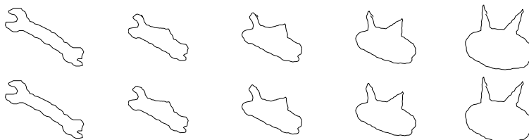
FIGURE 6. Curve evolution with and without the closedness constraint. Lower and upper bounds for the geodesic distance: 0.433 and 0.439
