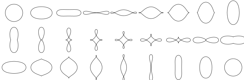
FIGURE 3. A great circle geodesic on B_{od} . The geodesic begins at the circle at the top left, runs from left to right, then to the second row and finally the third. It leaves B_{od} twice: at the top right and bottom left, in both of which the singularity of figure 1 occurs in 2 places. The index of the curve changes from +1 to -3 in the middle row. See text.
