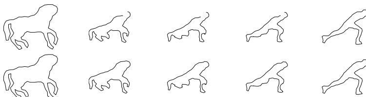
FIGURE 7. Curve evolution with and without the closedness constraint. Lower and upper bounds for the geodesic distance: 0.498 and 0.532
