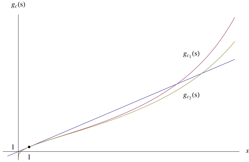
Figure 4: The functions g_{c_1}(s) and g_{c_2}(s) , for c_1 < c_2 .
