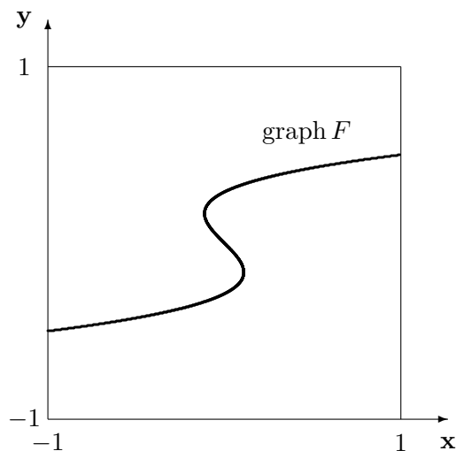
Figure 1: The graph of F
