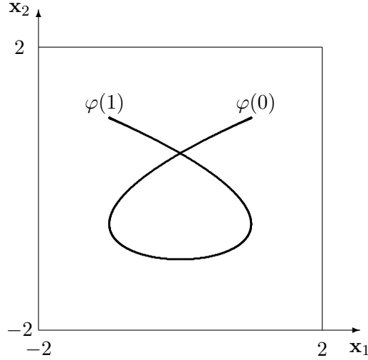
Figure 2: The projection of \text{Im } \varphi to \mathbf{x}
