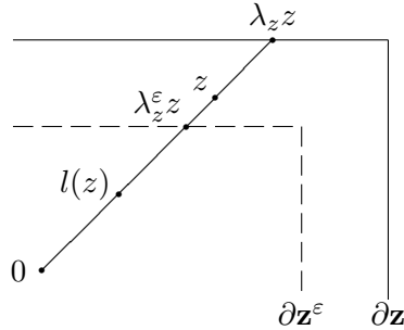
Figure 3: Illustration of the mapping l
