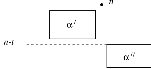
FIGURE 4. The block decomposition for \alpha \in \mathfrak{S}_n(132)
