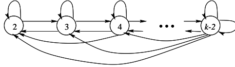
FIGURE 2. The directed graph for \mathcal{T}(123, (k-1, \dots, 2, 1, k))
