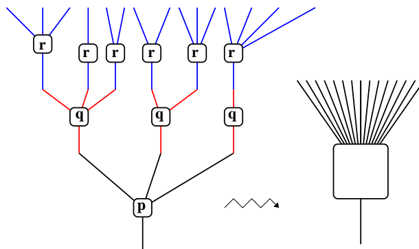
FIGURE 1. Main axiom for composition. First composing q 's and r 's then composing p and the result is the same as first composing p and q 's then composing the result and r 's. The common result is symbolically depicted on the right.
