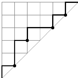
FIGURE 1. The Dyck path 01\ 001\ 011\ 01\ 01 \in \mathcal{D}_6 .
