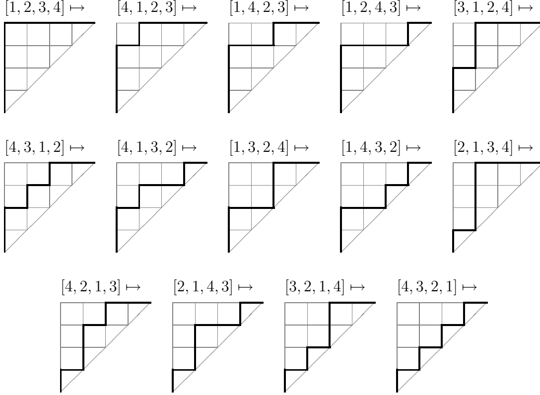
FIGURE 2. The bijection between \mathcal{S}_4(231) and \mathcal{D}_4 .
