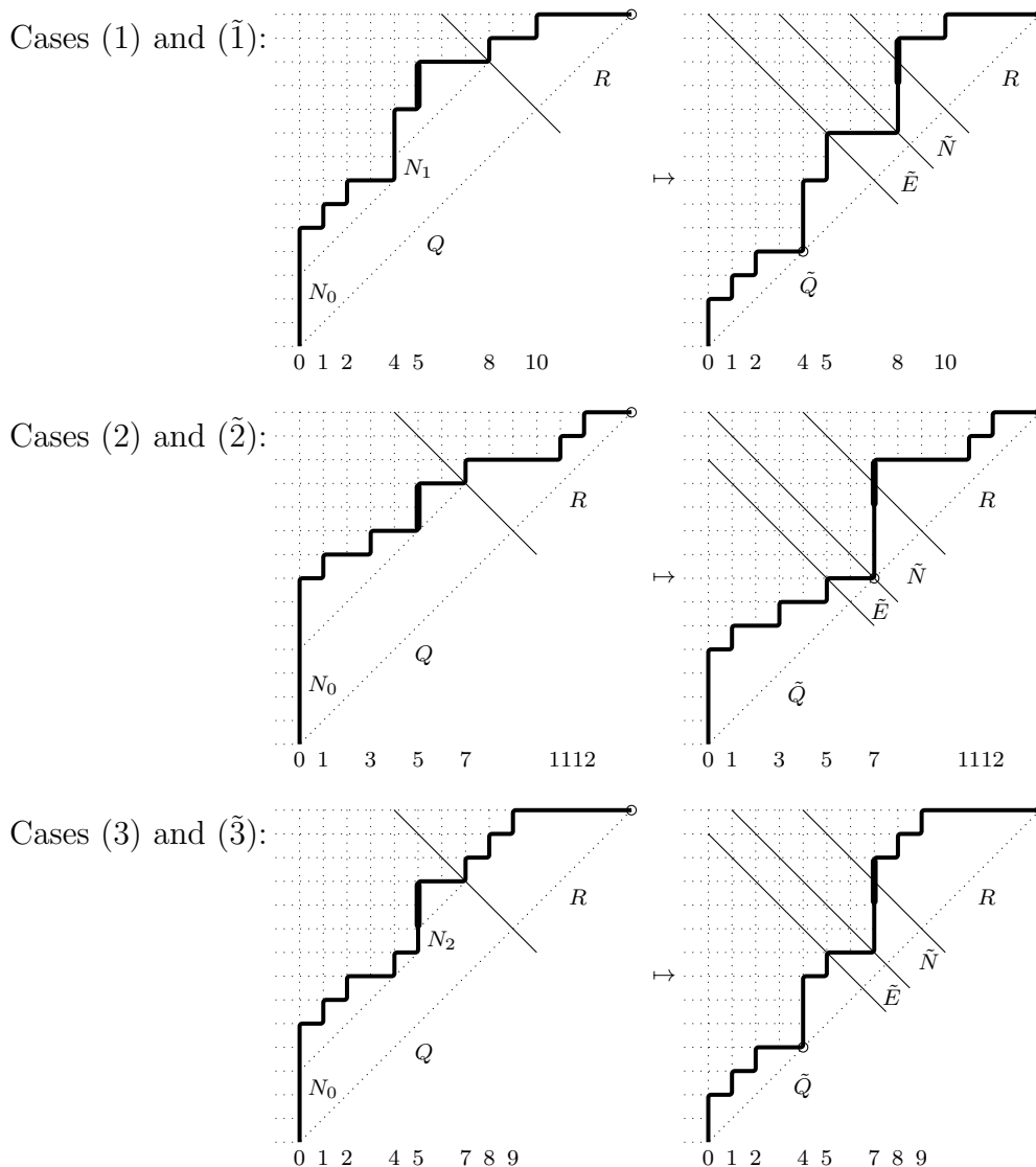
FIGURE 1. Examples for Dyck paths and their images under \phi
