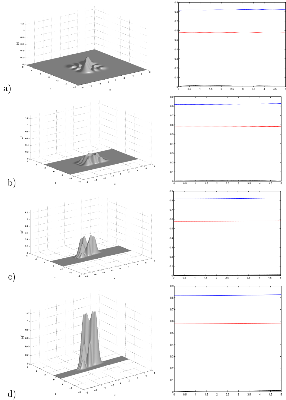
Figure 4: Surface plots (left column) of the position density |\psi^\varepsilon(x, t = 5)|^2 and the approximation errors \sigma_1^\varepsilon(t) (blue), \sigma_2^\varepsilon(t) (red), \sigma_3^\varepsilon(t) (black) (right column) for different \varepsilon : a) \varepsilon = 0.8 ; b) \varepsilon = 0.4 ; c) \varepsilon = 0.2 ; d) \varepsilon = 0.1 .
