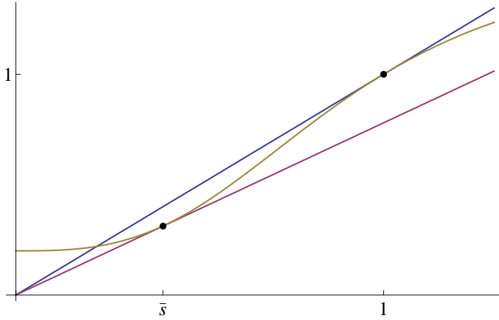
Fig. 2.2 Smooth pasting conditions for the function g , for \theta > 1 .
