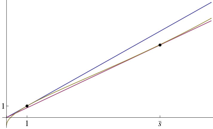
Fig. 2.1 Smooth pasting conditions for the function g .
