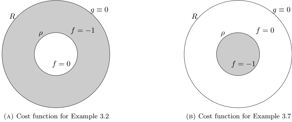
FIGURE 1. Cost functions for the examples of Section 3
