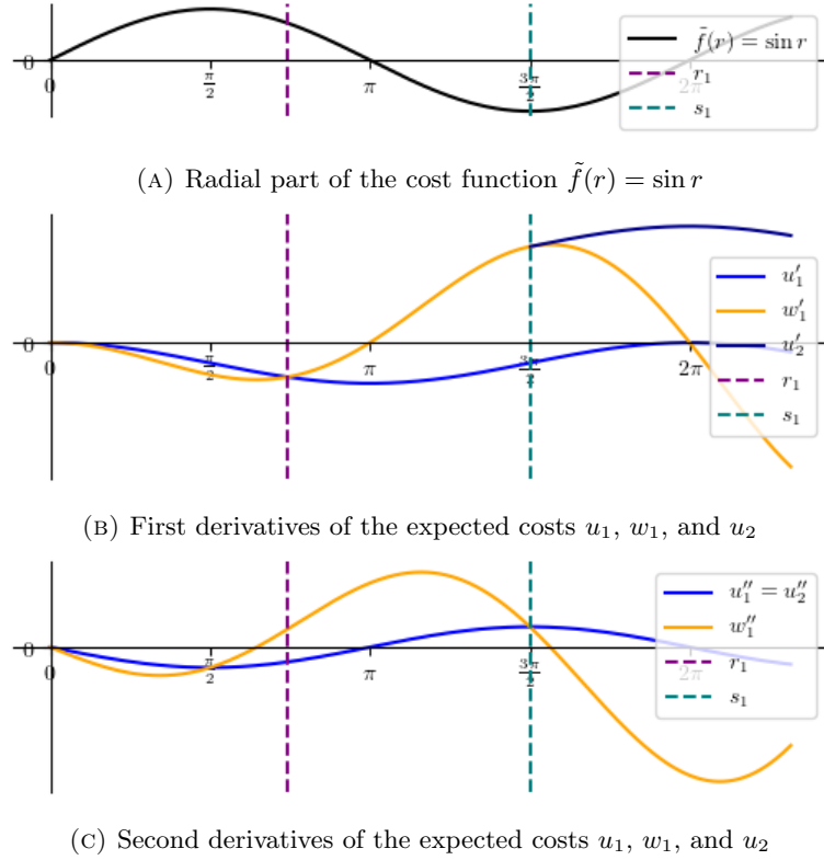
FIGURE 5. The first two switching points r_1 , s_1 are shown for the cost function f(x) = \sin |x| . The switching point r_1 is the first point at which w'_1(r) = -2r\tilde{f}(r) exceeds u'_1 , where u_1 solves u'_1(r) = -2\tilde{f}(r) , with u'_{1+}(0) = 0 , as shown in (B). The switching point s_1 is the first point after r_1 at which u''_2 = -2\tilde{f} exceeds w''_1 , as shown in (C). Fixing u'_2(s_1) = w'_1(s_1) , we see in (B) that s_1 is chosen such that u'_2 remains greater than w'_1 over an interval of positive length.
