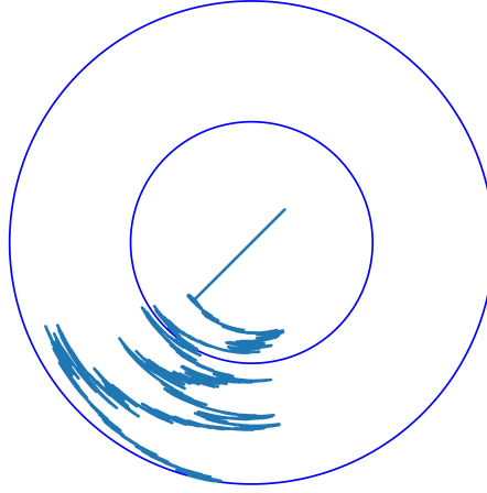
FIGURE 2. A possible trajectory for an optimal strategy in Example 3.2
