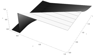
Figure 1.8. Rarefaction wave for Burgers' equation
