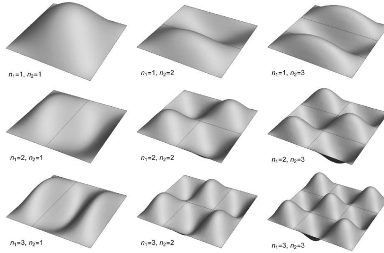
Figure 3.7. Fundamental tone and some overtones of a rectangular membrane
