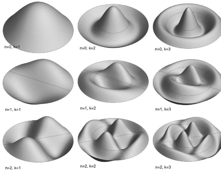
Figure 3.9. Fundamental tone and some overtones of a disc shaped membrane
