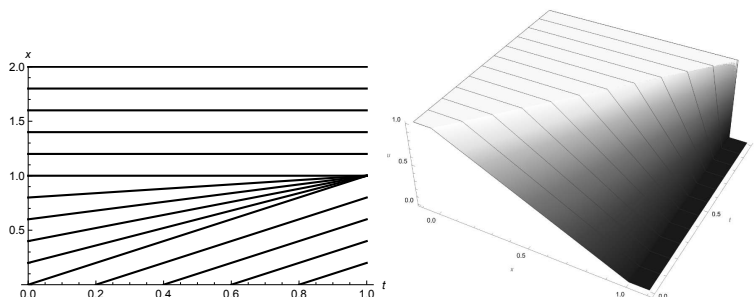
Figure 1.4. Shock wave for Burgers' equation: Characteristics (left) and solution (right) for steplike initial data
