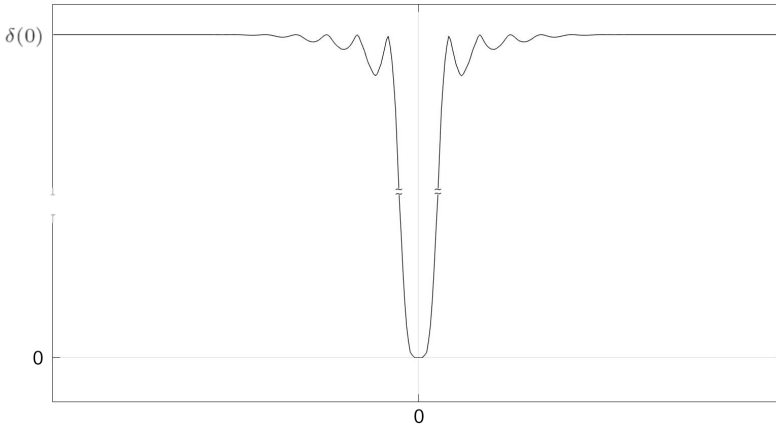
Fig. 4.2. A representation of \delta \circ \delta
