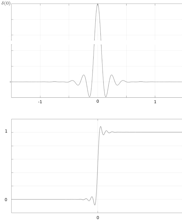
Fig. 4.1. A representation of Dirac delta and Heaviside function. A Colombeau mollifier has a representation similar to Dirac delta (but with finite values).
