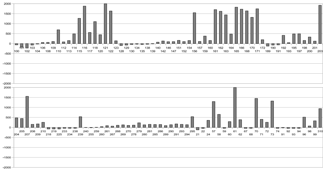
FIG. 25: Linearly constrained (variable box) — rp(c) for BNLC & SolvOpt ( T = |y|_2 )
