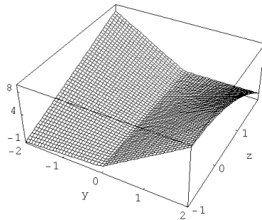
FIG. 12: f for (\mathbf{F}^2, T_1) \implies \hat{f} = -1
