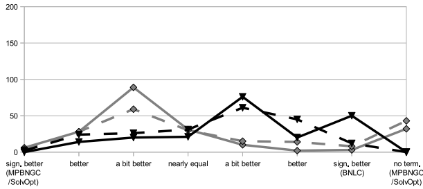
FIG. 17: Nonlinearly constrained (summary)
