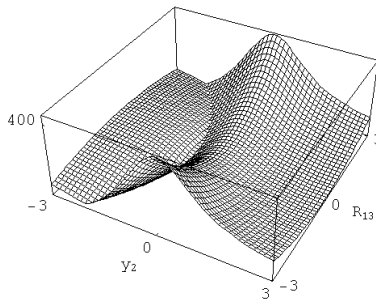
FIG. 6: f(y_2, R_{13}) for T_2
