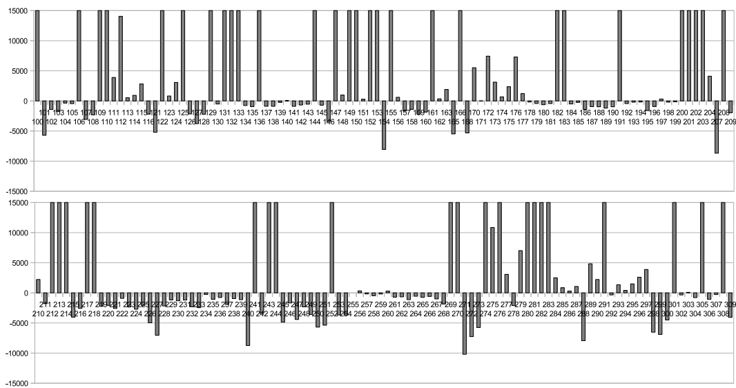
FIG. 27: Nonlinearly constrained — rp(c) for Red Alg & MPBNGC ( T = |y|_2 )
