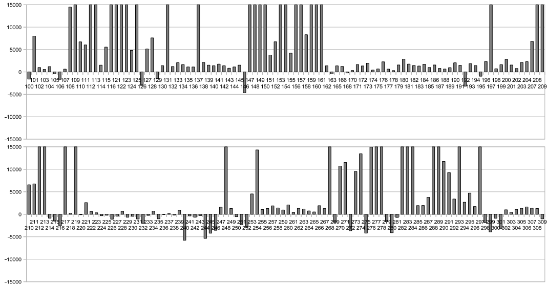
FIG. 28: Nonlinearly constrained — rp(c) for Red Alg & SolvOpt ( T = 1 )
