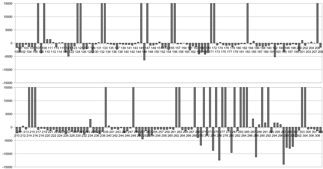
FIG. 26: Nonlinearly constrained — rp(c) for Red Alg & MPBNGC ( T = 1 )
