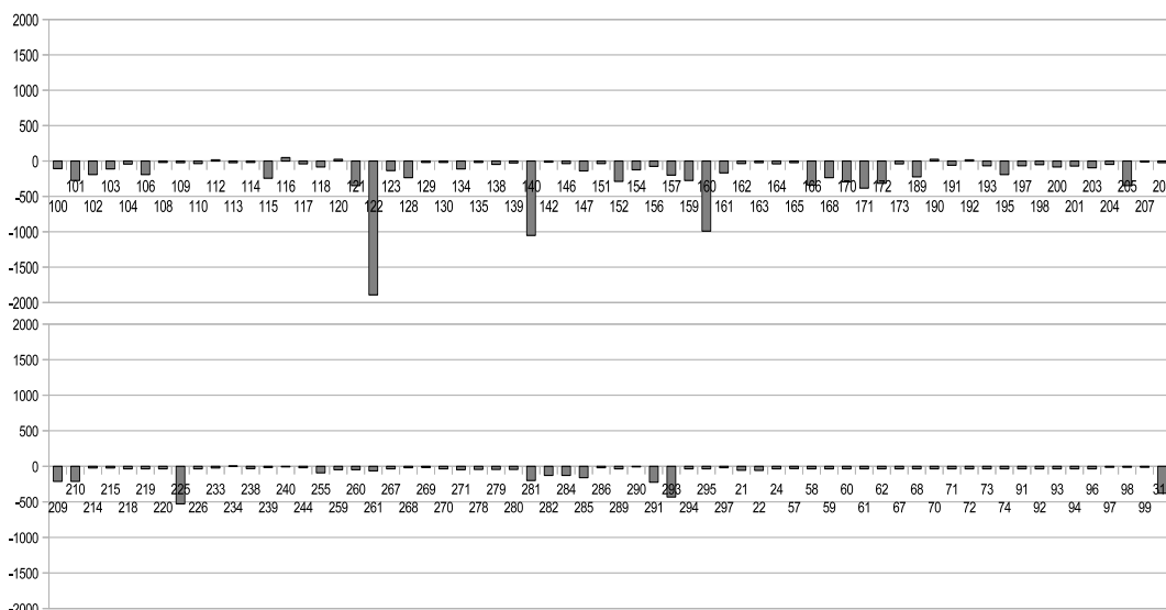
FIG. 19: Linearly constrained (fixed box) — rp(c) for BNLC & MPBNGC ( T = |y|_2 )
