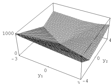
FIG. 1: f(y_1, y_2) for T_1
