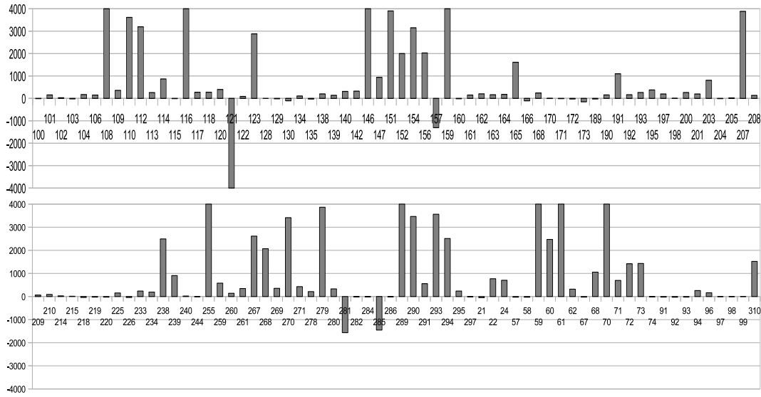
FIG. 20: Linearly constrained (fixed box) — rp(c) for BNLc & SolvOpt ( T = 1 )
