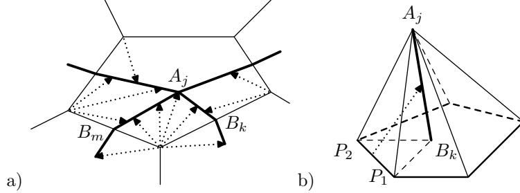
FIGURE 10. Proof of Lemma 2.8.
