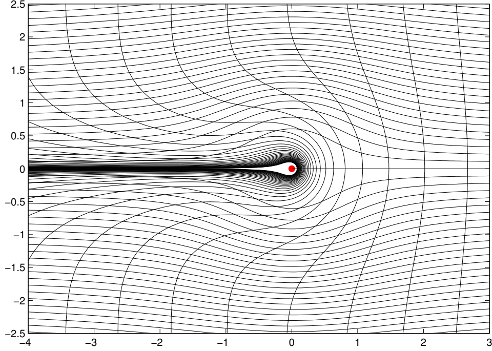
FIGURE 2. The result of the incompressible flow from t = -\infty to t = 0 with n = 2 , momentum concentrated at one point and K = K_{0,\eta} , \eta = .
