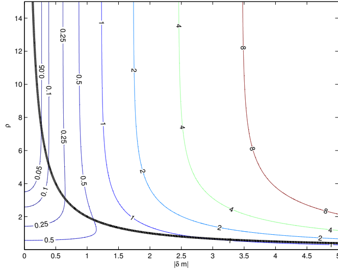
FIGURE 3. Level sets of energy for the collision of two vortons with \bar{m} = 0 , \eta = 1 , \omega = 1 . The coordinates are \rho = |\delta P| and |\delta m| , and the state space is the double cover of the area above and right of the heavy black line, the two sheets being distinguished by the sign of \langle \delta m, \delta P \rangle . The heavy black line which is the curve \rho \cdot |\delta m| = \omega where \langle \delta m, \delta P \rangle = 0 . Each level set is a geodesic. If they hit the black line, they flip to the other sheet and retrace their path. Otherwise \rho goes to zero at one end of the geodesic.
