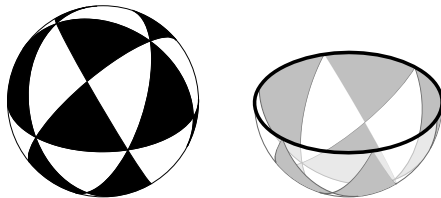
FIGURE 1. The Coxeter complex of type A_3 and one of its walls.
