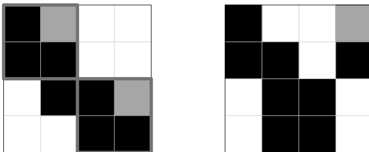
Figure 5: Left: Performing block lower triangular decomposition first, and then applying tearing to the two 2 \times 2 blocks on the diagonal leads to suboptimal results. The variables that have to be guessed in each block are marked gray. Right: The optimal ordering. The only guessed variable is marked gray.
