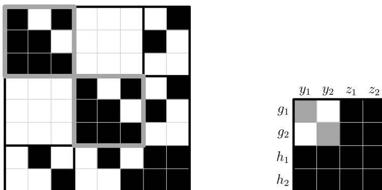
Figure 7: Left: The original 8 \times 8 system; tearing will be applied to the marked two 3 \times 3 blocks on the diagonal to get a sequence of two implicit equations. Right: The gray 1 \times 1 blocks are the result. This reduced 4 \times 4 system can be posed to a solver as the 2 \times 2 system h(z) = 0 by applying tearing again, and solving the implicit g_i for y_i ( i = 1, 2 ) internally.
