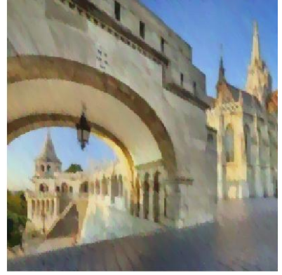
Figure 1: The original image, the noisy image (corrupted with Gaussian noise with standard deviation \sigma = 10 ) and the obtained reconstructed images for the choices (I)-(III) and a tolerance error of \varepsilon = 10^{-6}
