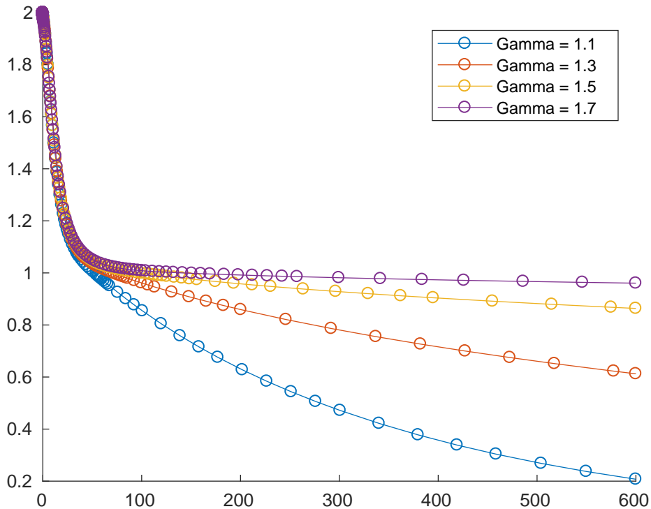
Figure 2: The behaviour of the trajectories generated by the dynamical system (5) in relation with the minimization of the function given in (6) for \alpha = 200 , \beta = 1 , \epsilon(t) = t^{-\gamma} and different values for \gamma \in (1, 2) .
