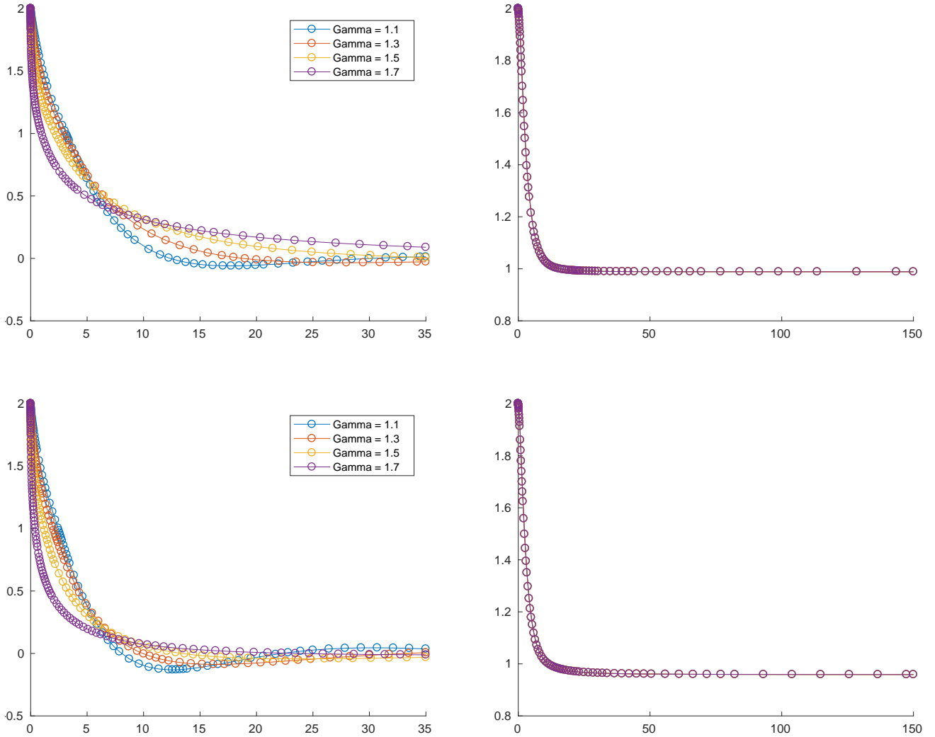
Figure 1: First column: the trajectories of the dynamical system with Tikhonov regularization \epsilon(t) = t^{-\gamma} are approaching the minimum norm solution x^* = 0 . Second column: the trajectories of the dynamical system without Tikhonov regularization the trajectory are approaching the optimal solution 1.
