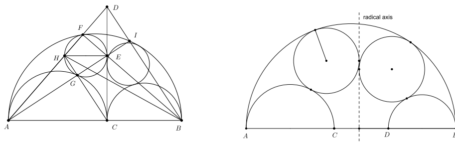
Figure 2: Archimedes' proof of Proposition 5 (left); Our sketch belongs to the generalized version of Proposition 5 (right)
