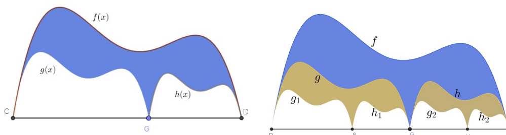
Figure 6: The f-belos(left), two more f-belos (right).
