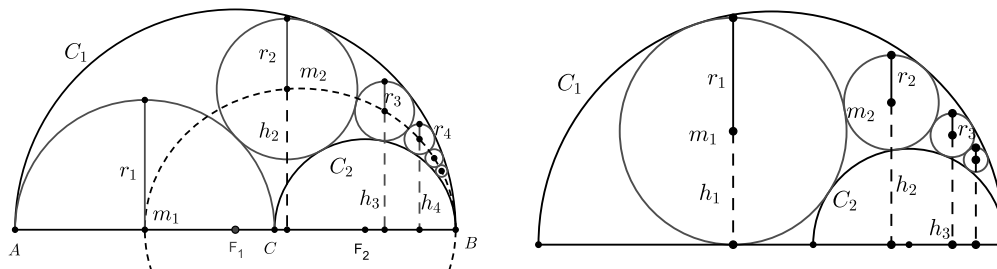
Figure 4: Pappus' Props. 16 (left); Pappus' Props. 18 (right).
