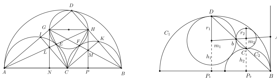
Figure 3: Archimedes' proof of Proposition 6; GH = NP = \frac{6}{19}AB (left); The "ancient theorem" of Pappus, Pappus' Prop. 15, (right).
