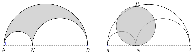
Figure 1: The arbelos (left); The area of the circle with diameter PN is equal to the area of the arbelos (right).
