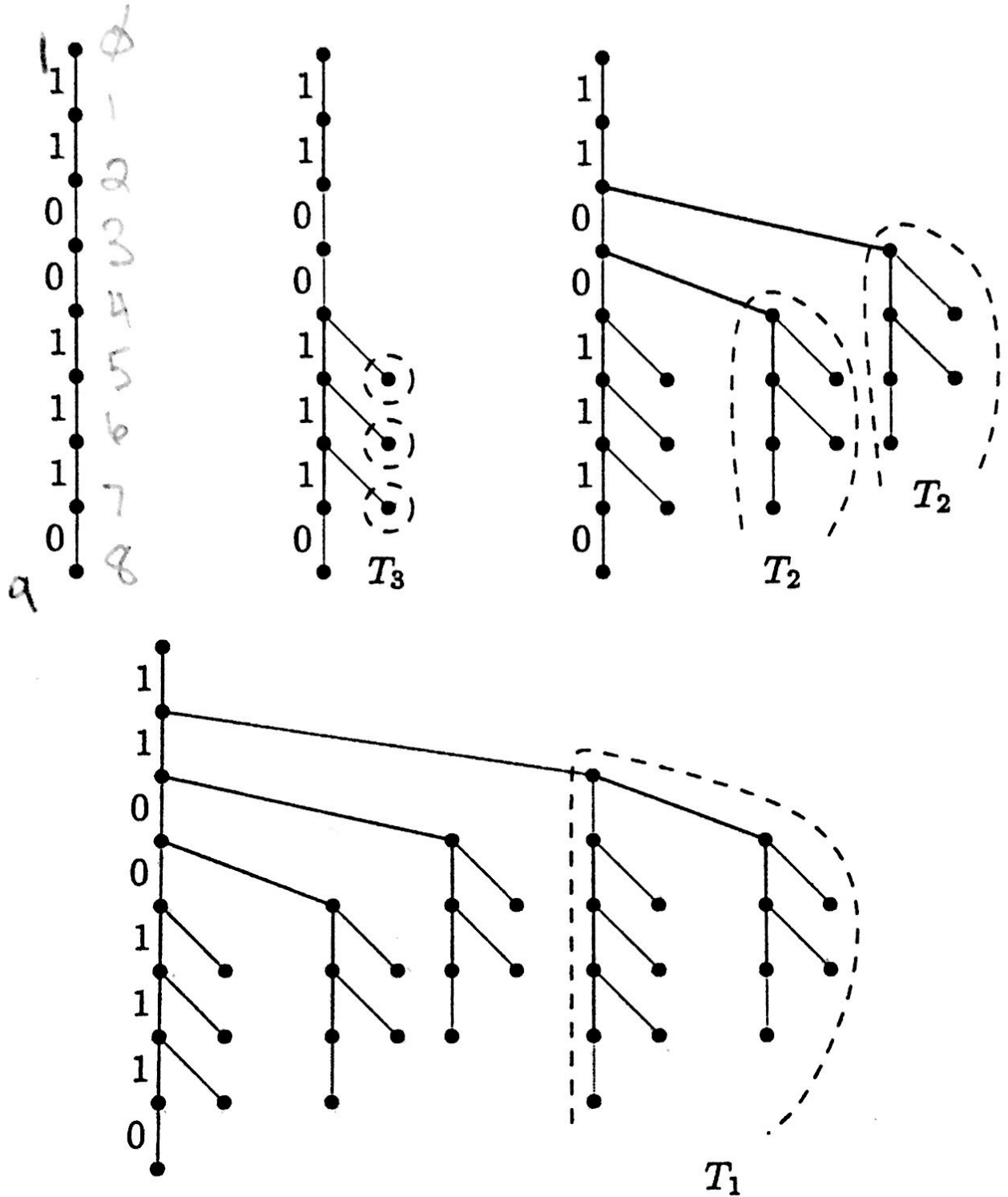
Fig. 4. Bottom-up construction of \tau_{L_2}(11001110) .
