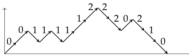
Figure 1: Example of a weighted Dyck path in DW_{14} .
