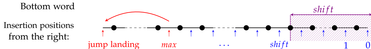
Figure 3: Insertion positions in the building bottom word (dots are word's elements).
