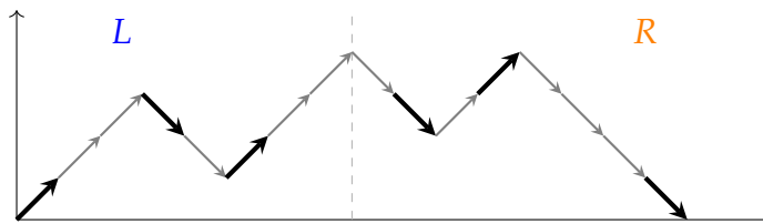
Figure 4: Locations where the jump is decided using the peak or valley condition.
