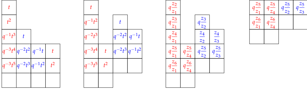
Figure 1: (\delta^S, f_S^{\text{st}}) , (\delta_S, f_S) , (\delta_S, f_S^z) and (\text{Rec}^{\leq m}, g_S)
