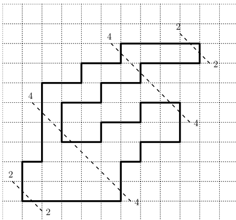
FIGURE 2. Showing the decomposition of an imperfect staircase polygon into a sequence of 2-4-2 non-intersecting walkers, each expressible as a Gessel-Viennot determinant
