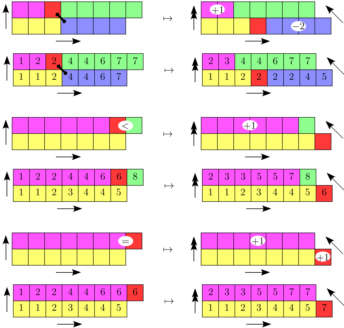
Figure 2. The three cases of the bijection, from a Magog trapezoid to a Gog trapezoid. On the top line, the first bug is 3: it is symbolized by a small black diagonal line. The colored blocks are moved and, whenever there is a tag on a block, it is added to all the elements of the block.
