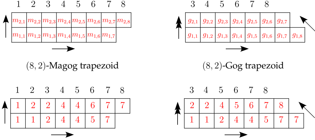
Figure 1. The conditions satisfied by (n, 2) -Magog and Gog trapezoids. Every sequence formed by numbers obtained by following the direction of a simple-arrowhead (respectively a double-arrowhead) arrow is non-decreasing (respectively increasing).
